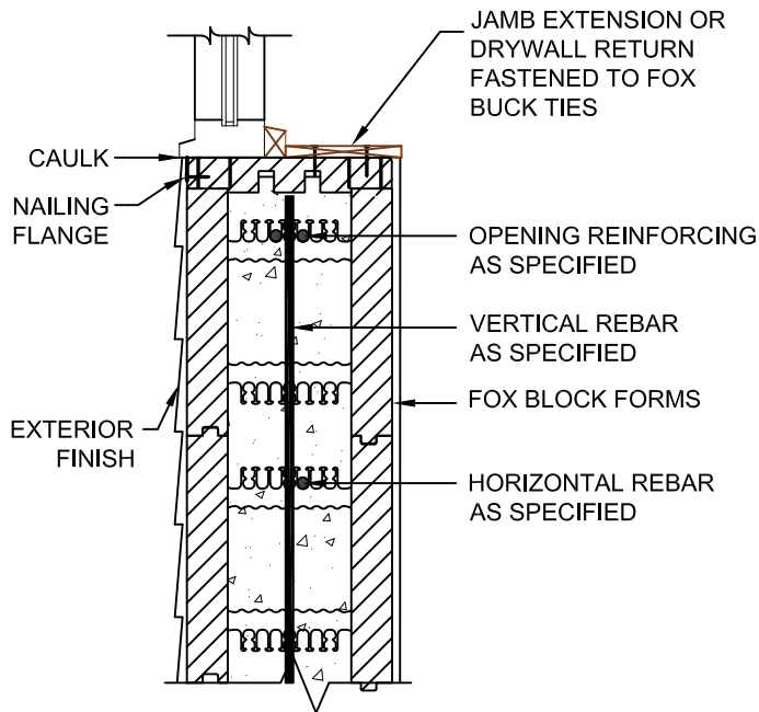
① SILL AND HEADER DETAIL
